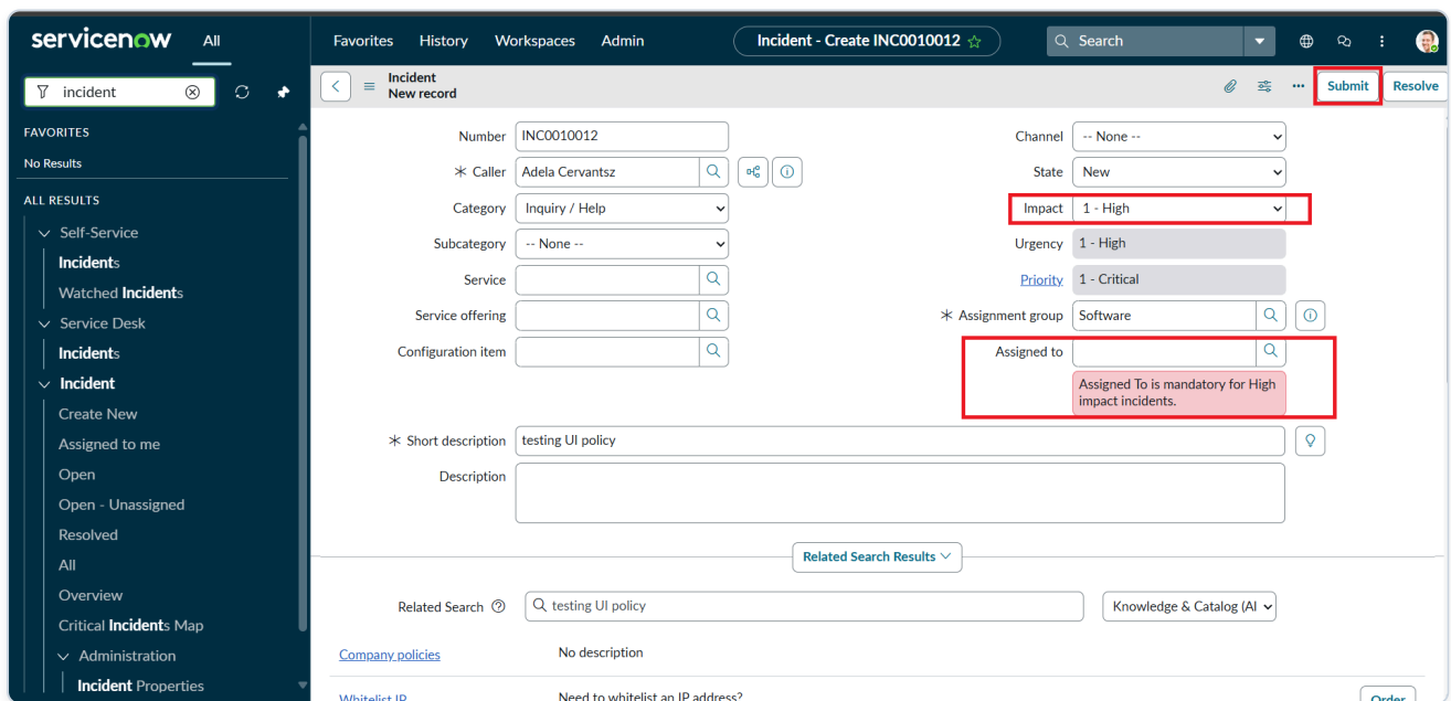
Figure 7.10: Test Activity 1 – Field-Level Red Error Box Rendered Below Assigned To
